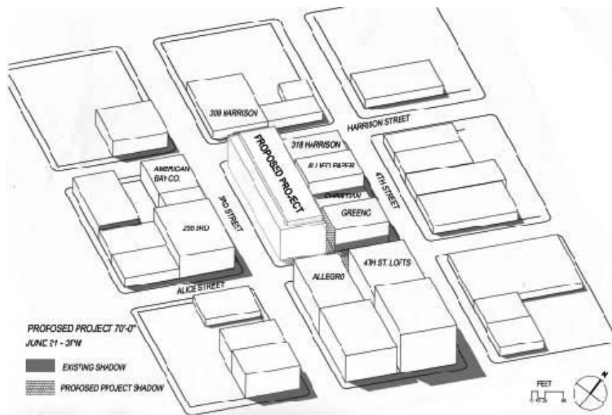
SHADOW ANALYSIS: JUNE 21
