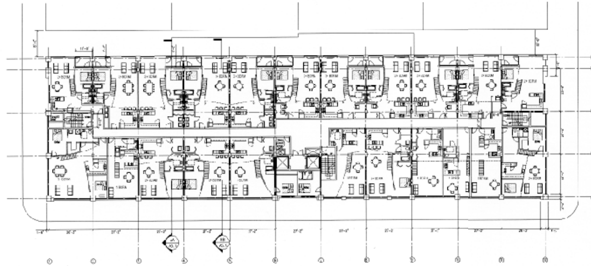
FOURTH LEVEL AND FOURTH LEVEL MEZZANINE PLANS
