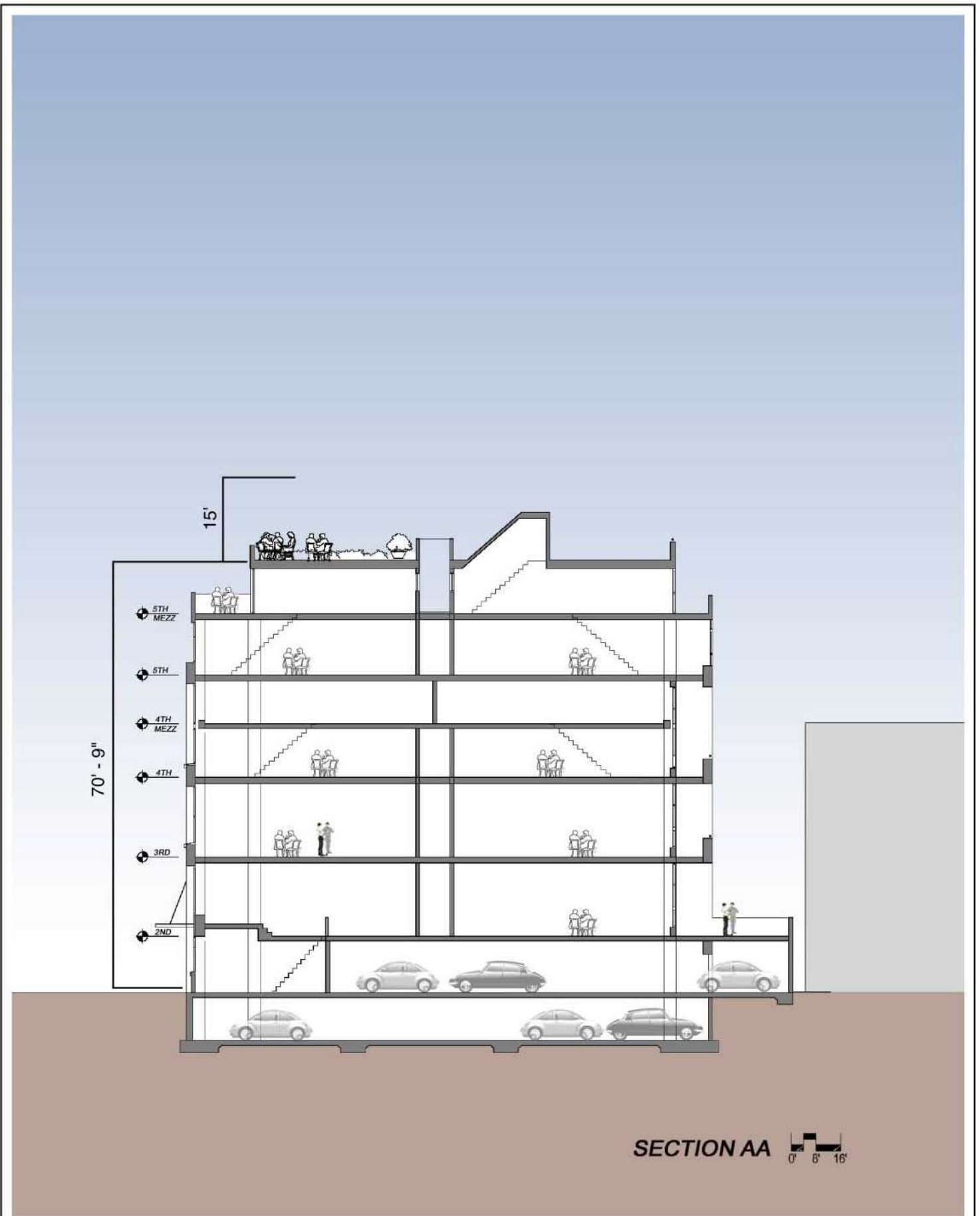
BUILDING CROSS-SECTION
