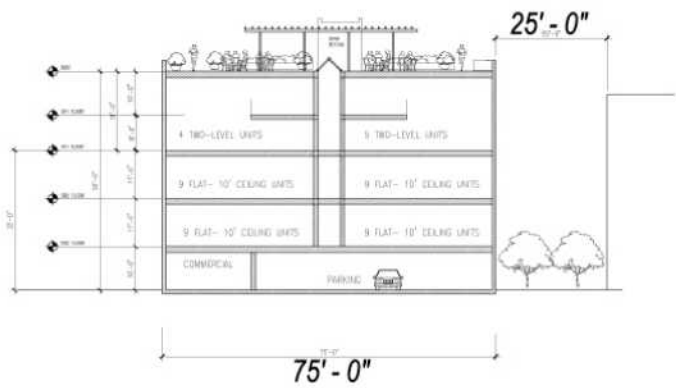
SECTION THRU 50' HIGH BLDG
